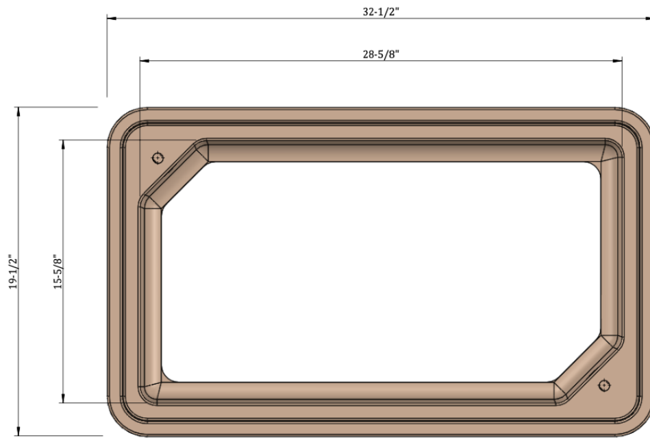
TOP VIEW OF BOX
