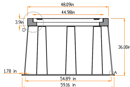
CROSS SECTION A-A'
